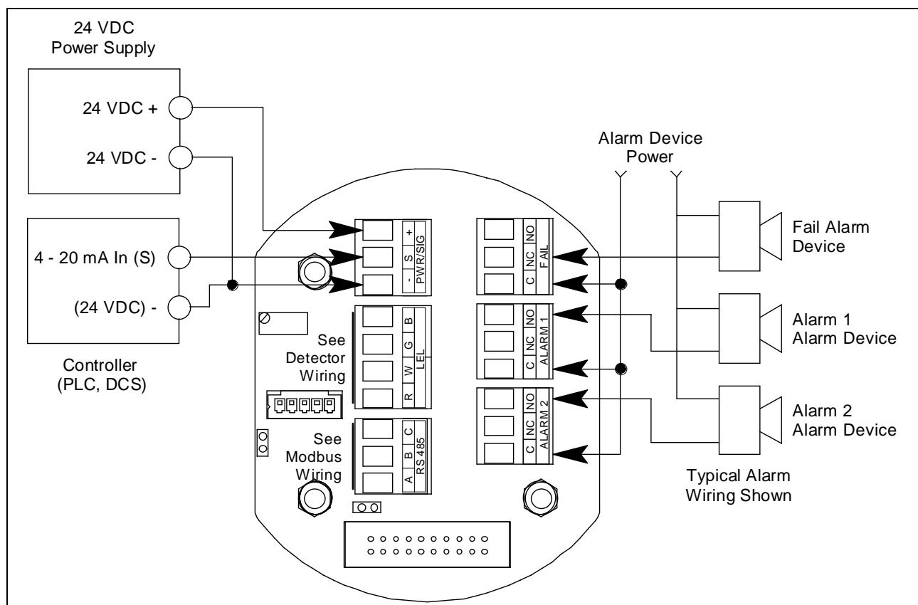
Figure 36: PLC and DCS Device Wiring
