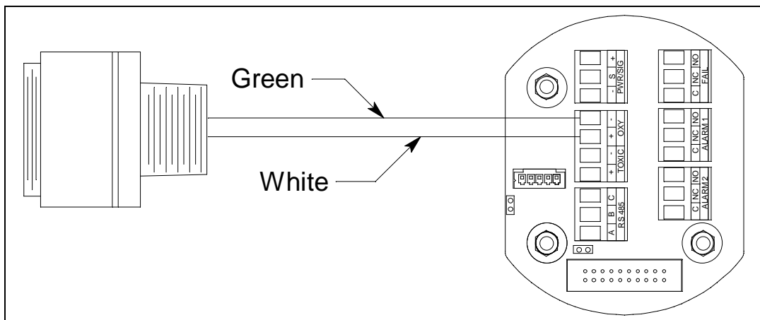
Figure 25: Capillary Type Replaceable Sensor Oxygen Detector Wiring
