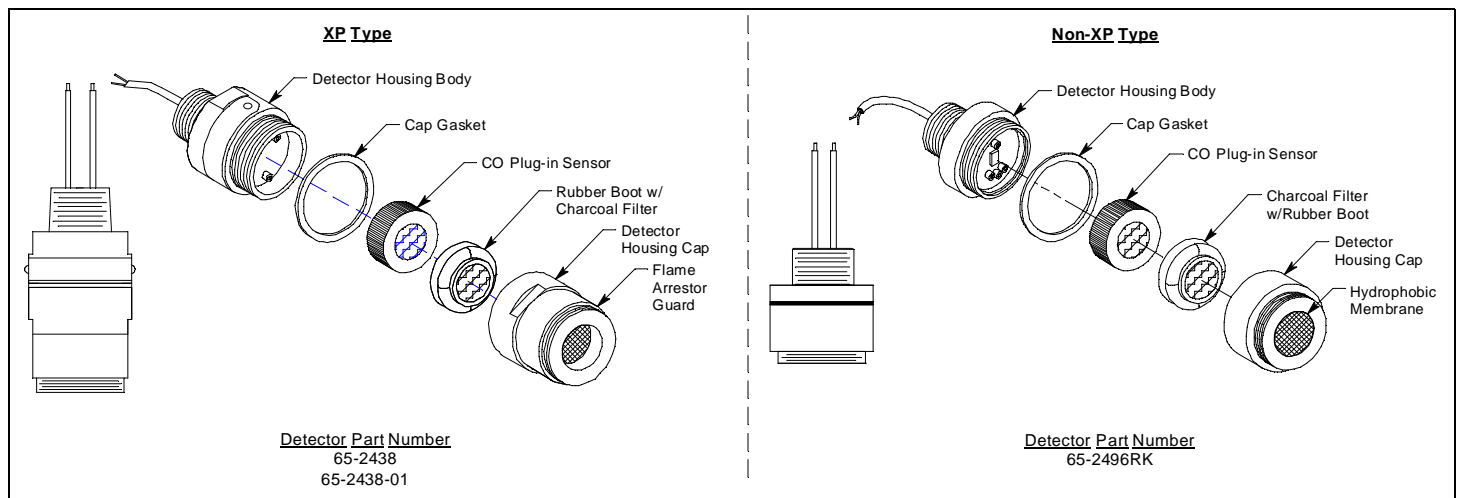
Figure 6: CO Detectors
