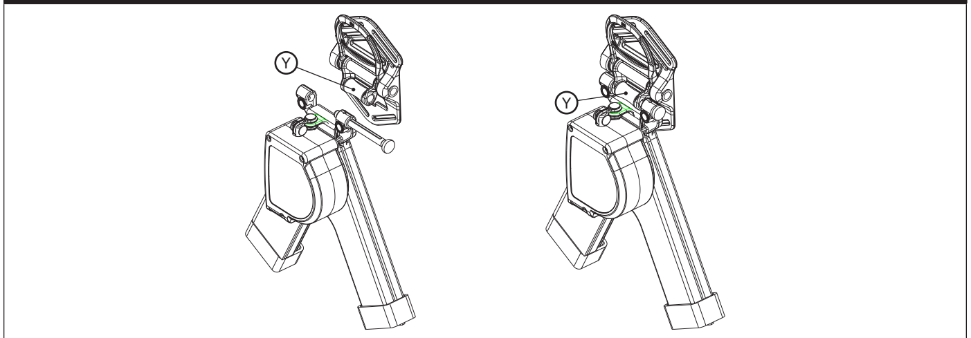
Figure 13 - SRD Adapter
