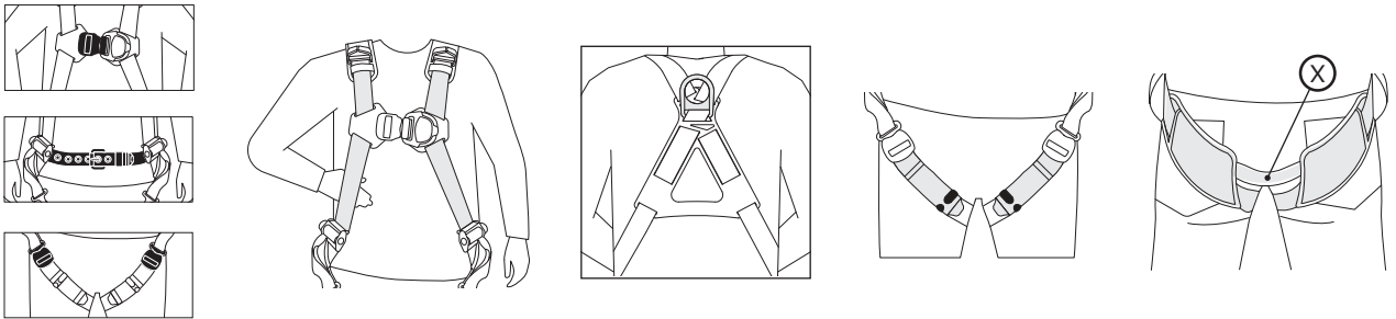
Figure 7 - Equipment Check
