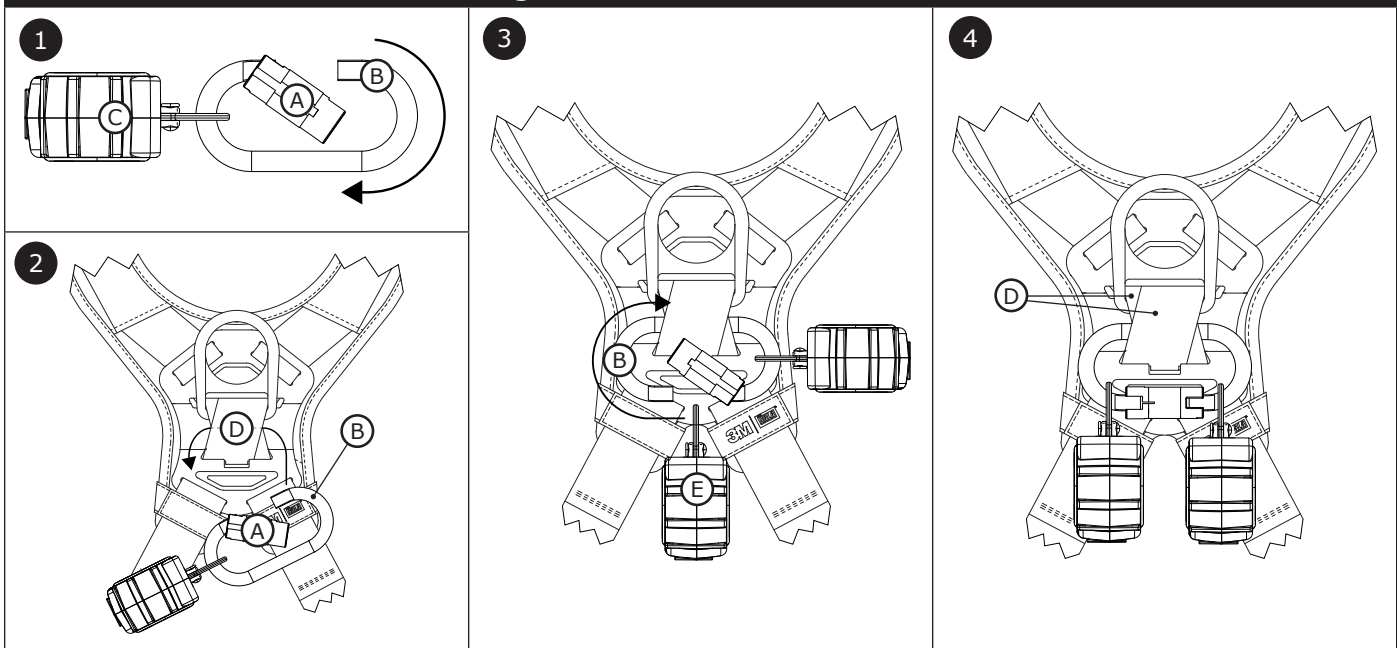
Figure 11 - Carabiner Interface
