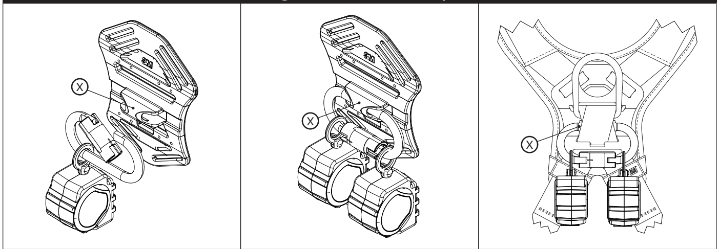
Figure 12 - Interface Loop
